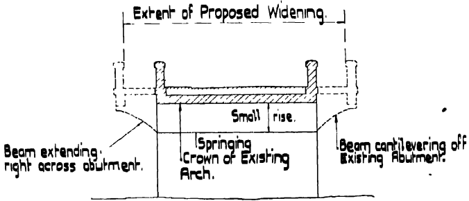
Fig. 208.—Widening by Double Cantilever resting directly on existing Pier.
